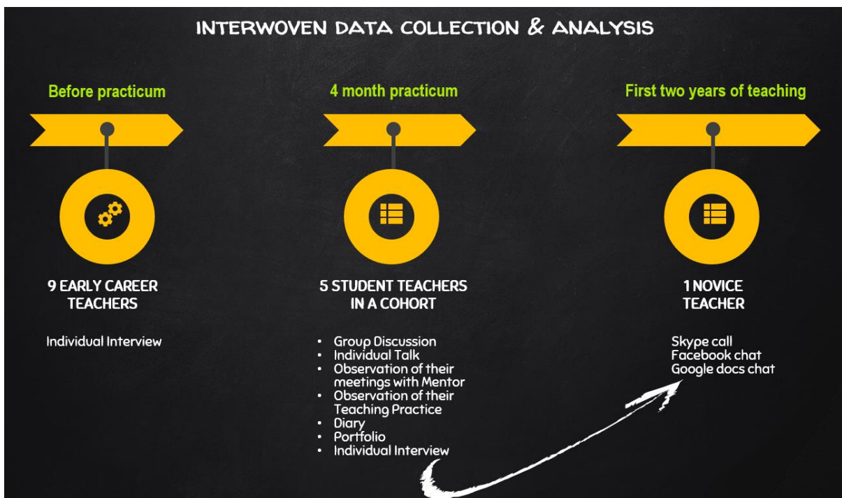
Figure 6 – Three stages of data collection and analysis reported in this thesis
