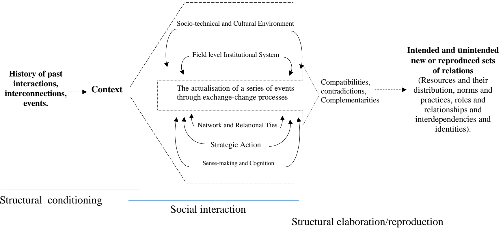
Figure 3 Analytical Framework
