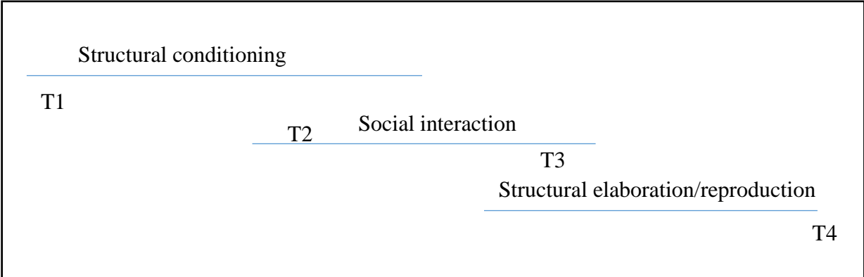
Figure 2 Morphogenetic-static cycle
