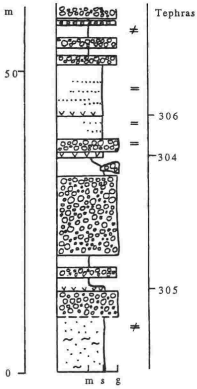
Fig. 2.5 Lithological column for Tukituki Road
