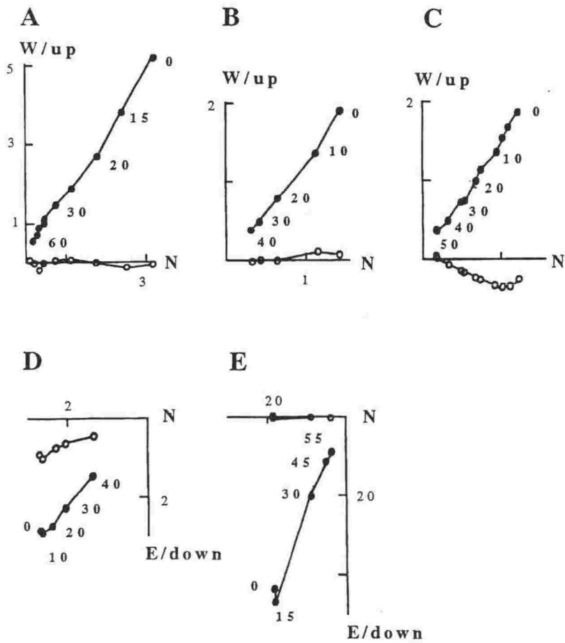
Fig. 3.2 Examples of demagnetisation behaviour of specimens with a single component magnetisation, plotted on orthogonal component diagrams. Solid dots represent the x and z components and open dots represent the x and y components. A= Mangatewainui site 4; B= Mangatewainui site 1c; C= Mangatewaiiti site 1c; D= Mangatewaiiti site 2c; and E= tephra 291, Vinegar Hill Rd.
