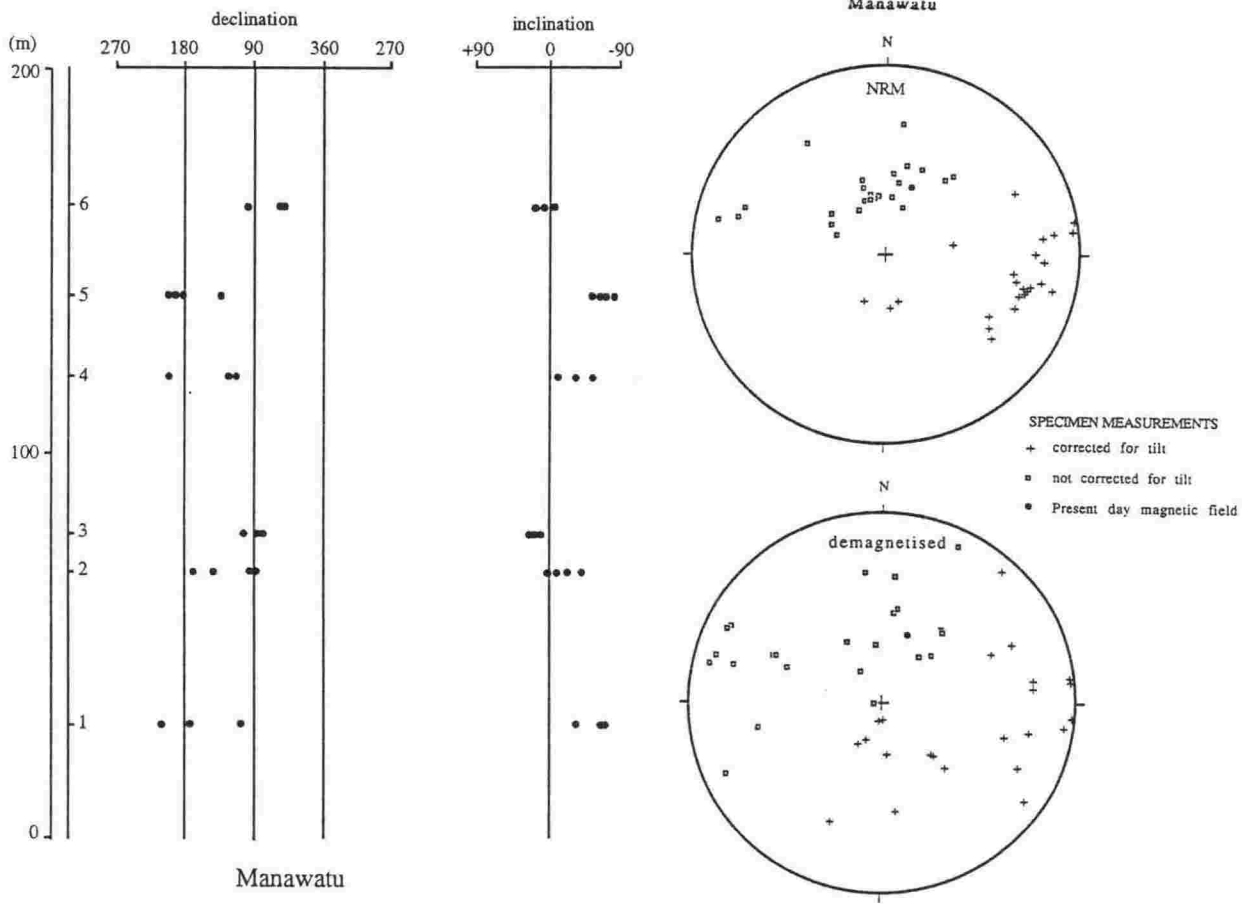
Fig. 3.11 Paleomagnetic specimen measurements for the Manawatu section. Plotted as in Fig. 3.6.
