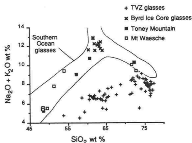
Fig. 5. Composition of SPTZ glasses compared to contemporaneous rocks and glasses from Antarctic volcanoes and the Taupo Volcanic Zone. Analyses for Toney Mountain from LeMasurier et al. (1990), Mt Waesche from LeMasurier and Kawachi (1990) and Byrd Ice Core from Palais et al. (1988)
