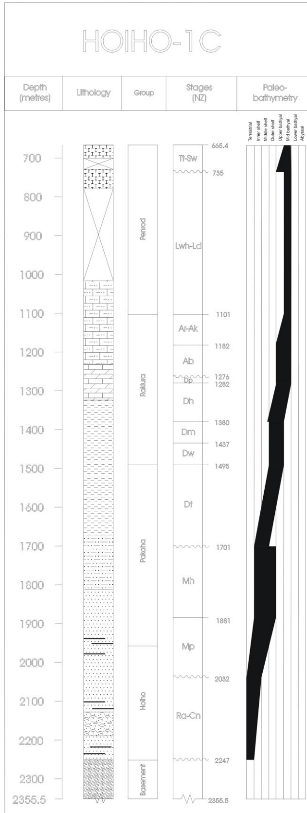
Figure 5.3: Stratigraphic column for Hoiho-1C, typical of the Great South Basin, New Zealand.
