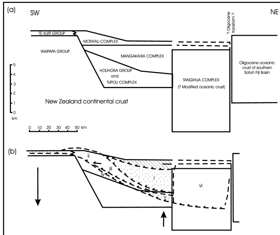
Figure 9.7: Schematic cross-section through northern Northland, showing inferred origin of nappes involved in the Allochthon movement. (From Brook and Hayward, 1989).
