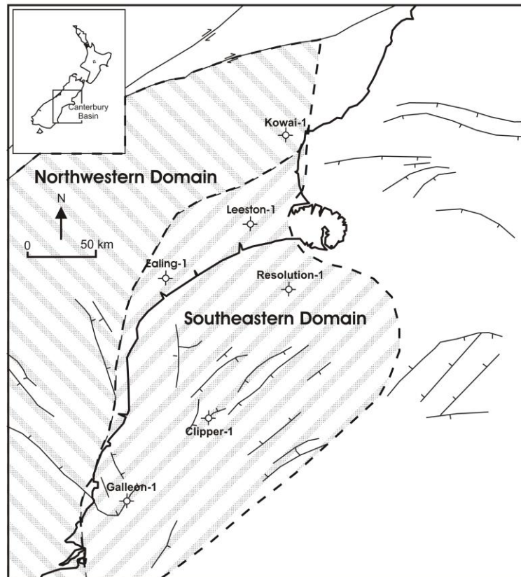
Figure 4.12: Oligocene and Neogene tectonic domains (After Field and Browne, 1993)
