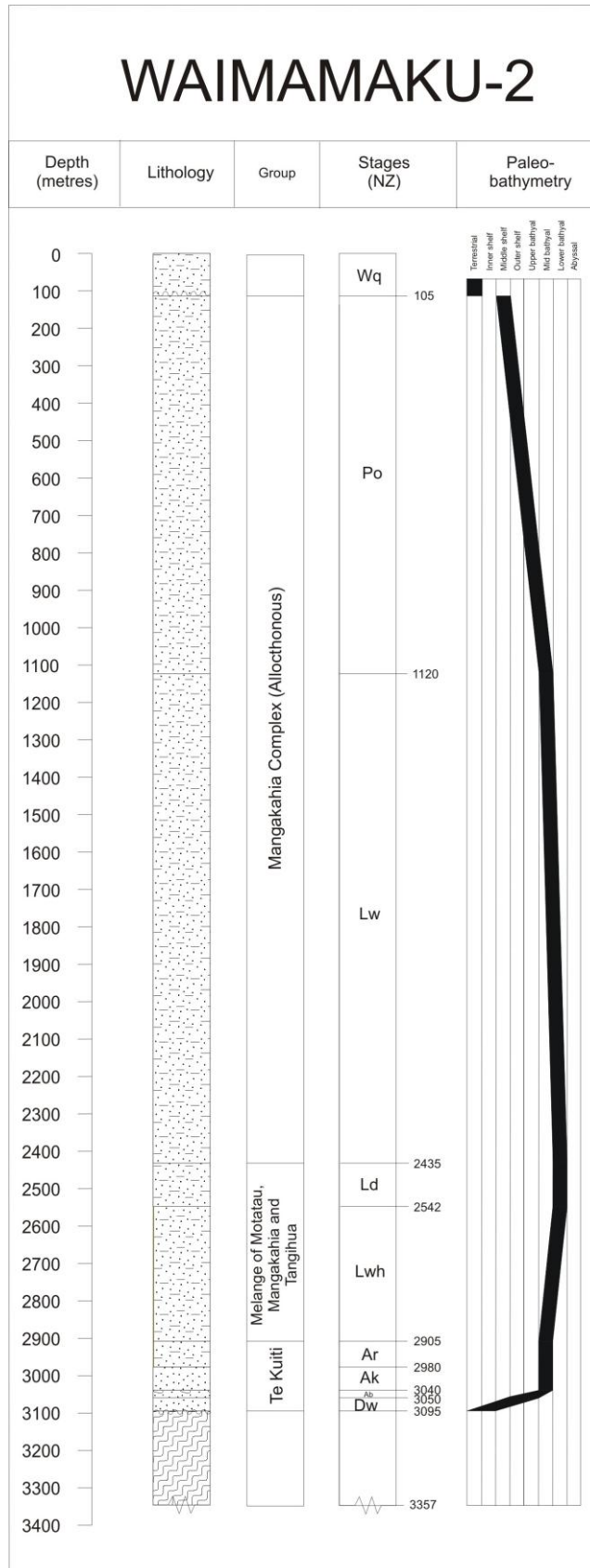
Figure 9.3: Stratigraphic column for Waimamaku-2, typical of the allochthonous region of Northland, New Zealand.
