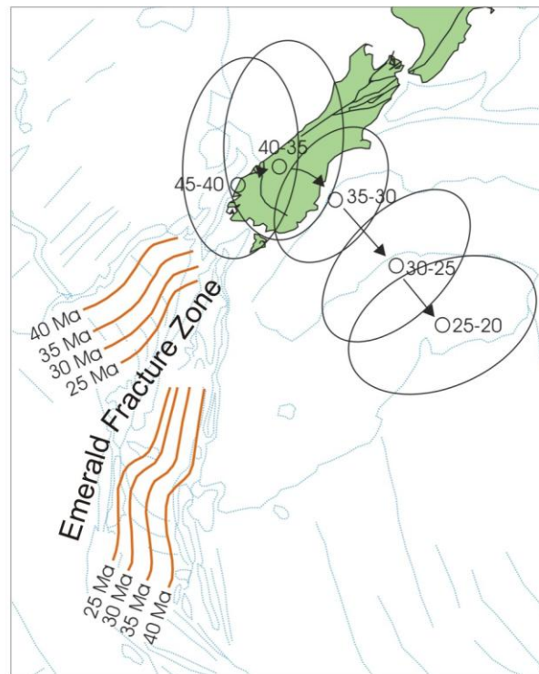
Figure: 5.8: Movement of the Australia-Pacific instantaneous pole with time (GEOS-NZ results 45-20 Ma; GEOS-3P results 20-0 Ma) and estimated isochrones for ocean crust south of New Zealand. (From Sutherland, 1995).
