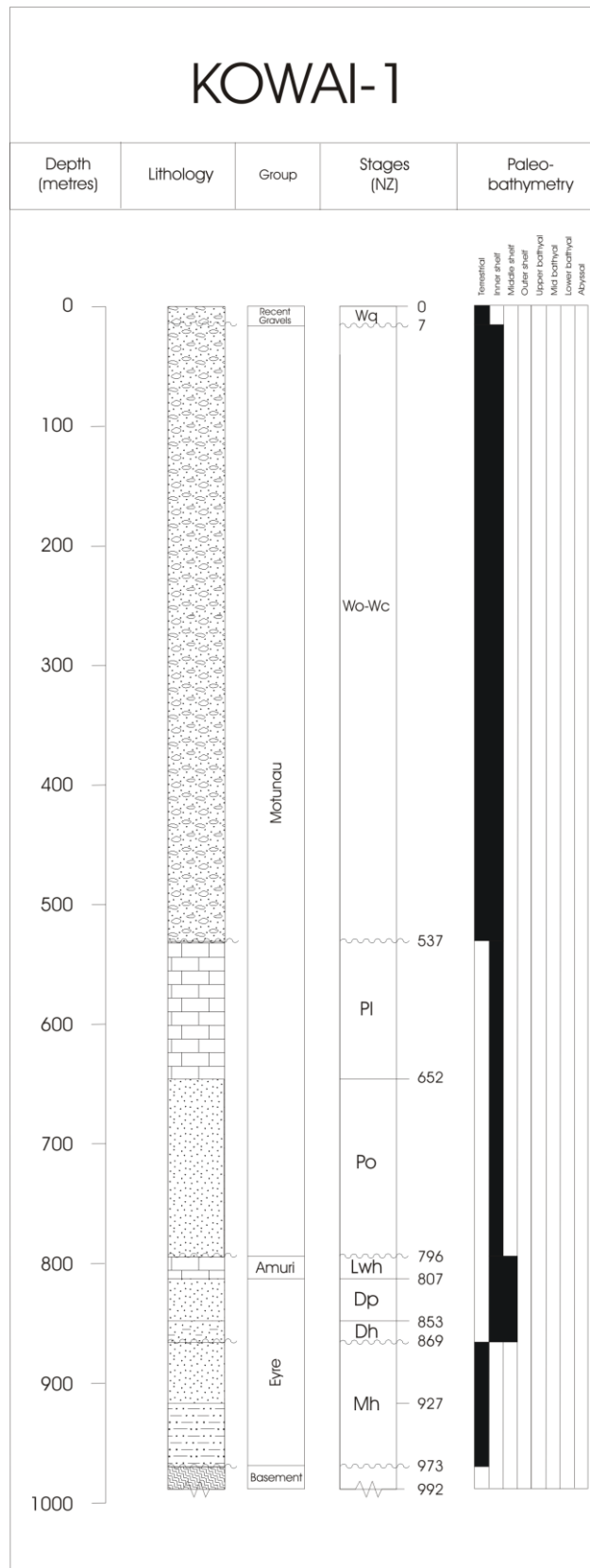
Figure 4.3: Stratigraphic column for Kowai-1, typical of Northern Canterbury, New Zealand.
