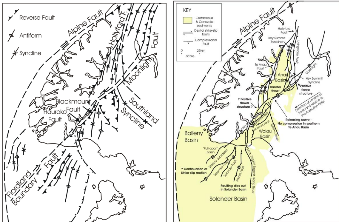
Figure 6.8: Map of Western Southland showing (a): location of antiforms and synforms during the Miocene (From Norris and Turnbull, 1993). (b): active faults, and the presence of restraining curves and pull apart basins (From Turnbull and Uruski et al., 1993)
