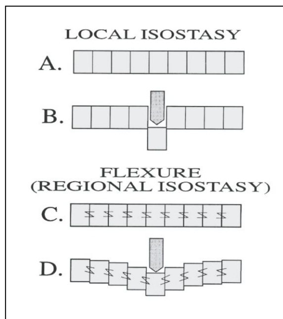
Figure 2.3: Comparison of local isostasy versus flexure (regional isostasy). In local isostasy (A), the lithosphere is composed of separate blocks. As a load is placed on the surface of the earth (B), only the block immediately beneath the load subsides. In reality the earth has lateral strength (C), as if the blocks are attached to each other by springs. Emplacement of a load on the surface causes subsidence (D), but is compensated over a larger area due to the rigidity of the lithosphere.
