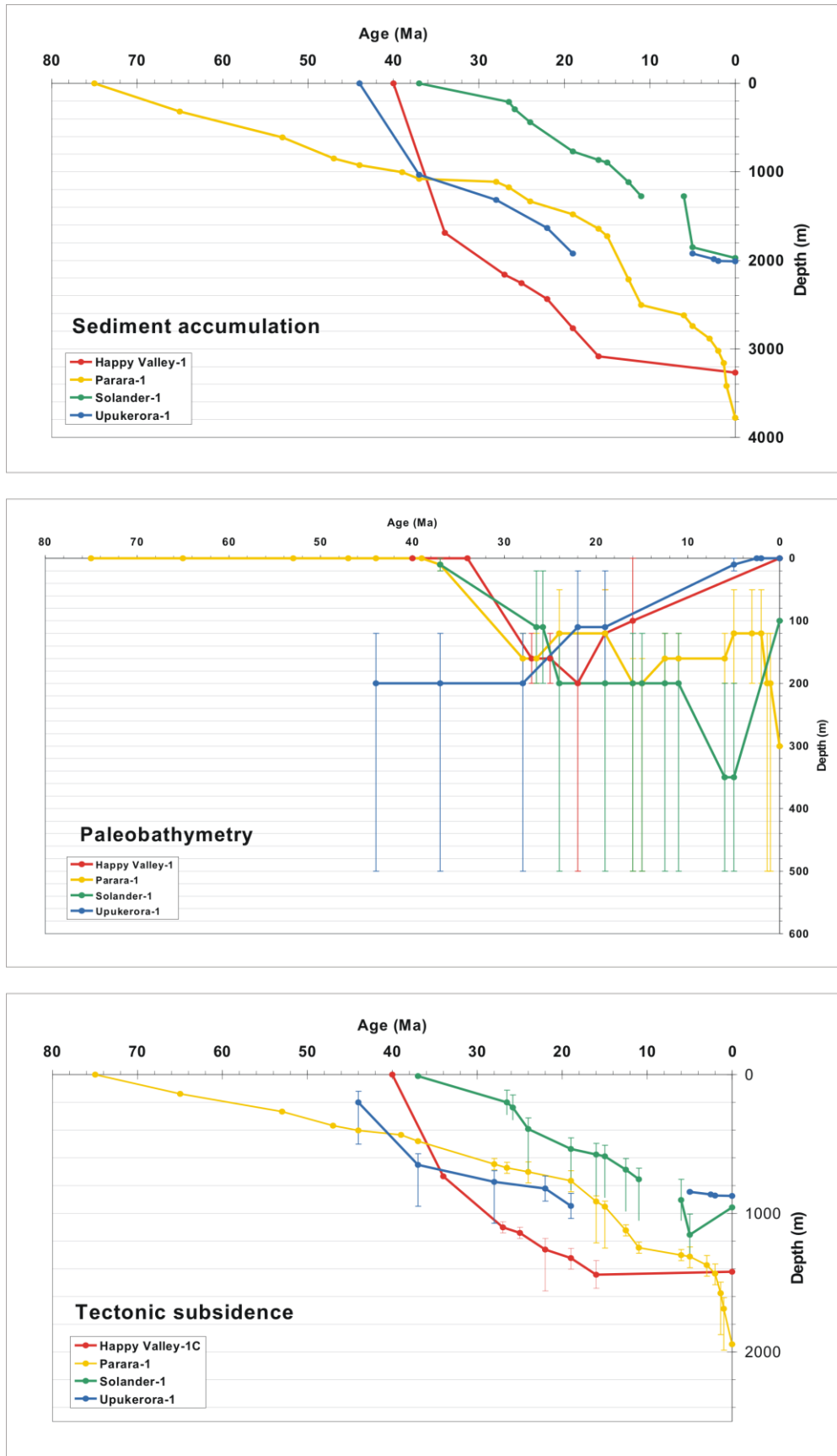
Figure 6.4: Geohistory plots for the wells located in the Western Southland Basins.
