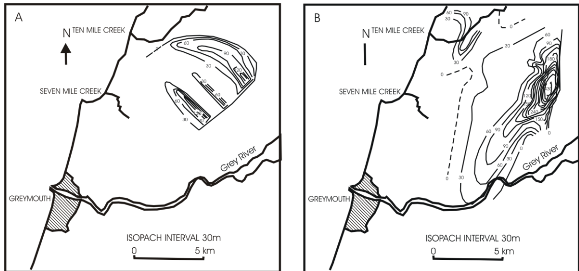
Figure 7. 10: Map of the Greymouth region showing the change in faulting trends seen with the help of isopachs during the deposition of the Paparoa Coal Measures (From Laird, 1993). A Isopach showing mid Cretaceous sedimentation of the Paparoa Coal Measures B Isopachs show a change in deposition and faulting, which occurred during mid-late Cretaceous.
