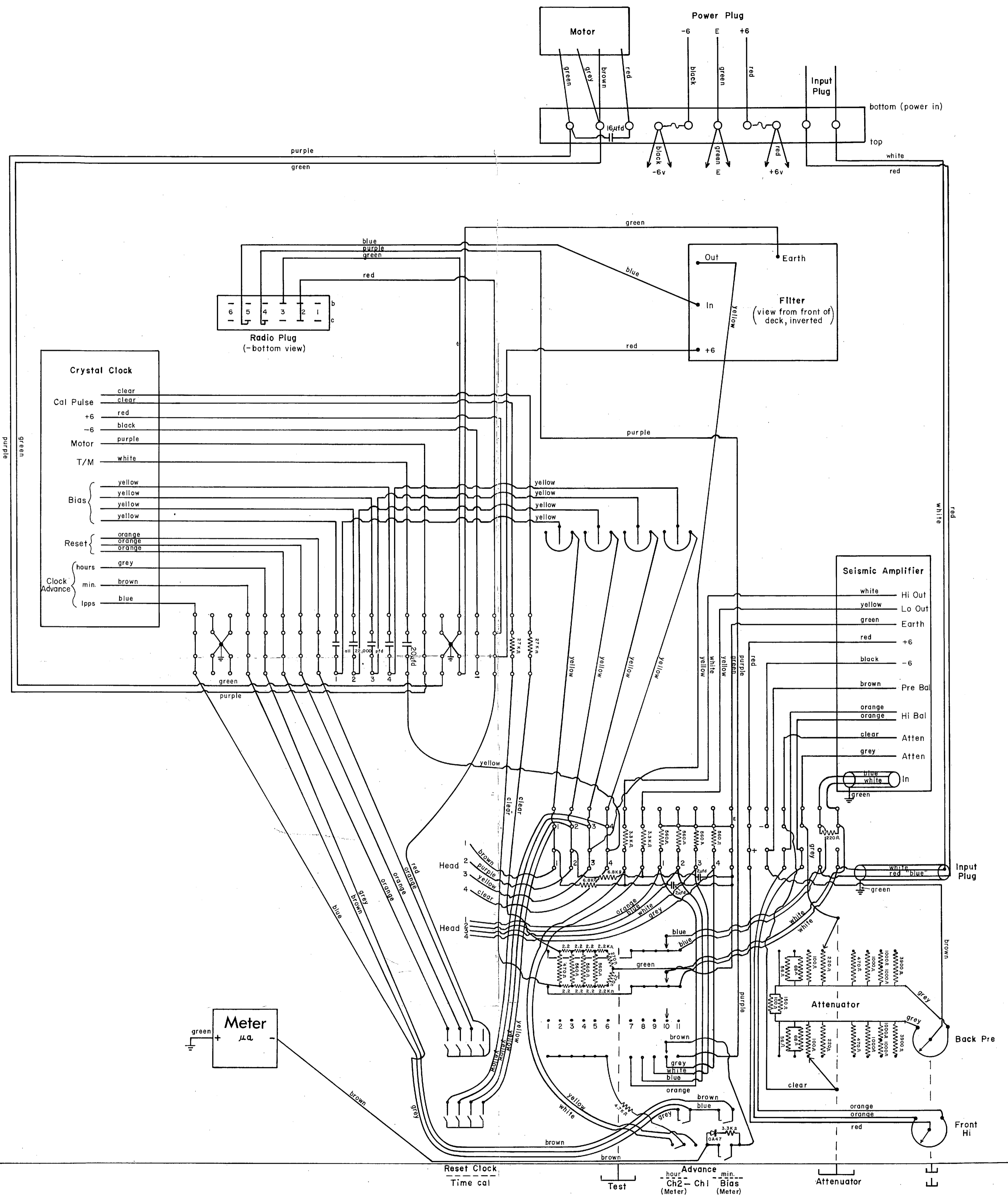
VIEW OF FRONT INVERTED FIG 2.8 WIRING DIAGRAM OF TAPE SEISMOGRAPH 1970 MODEL
