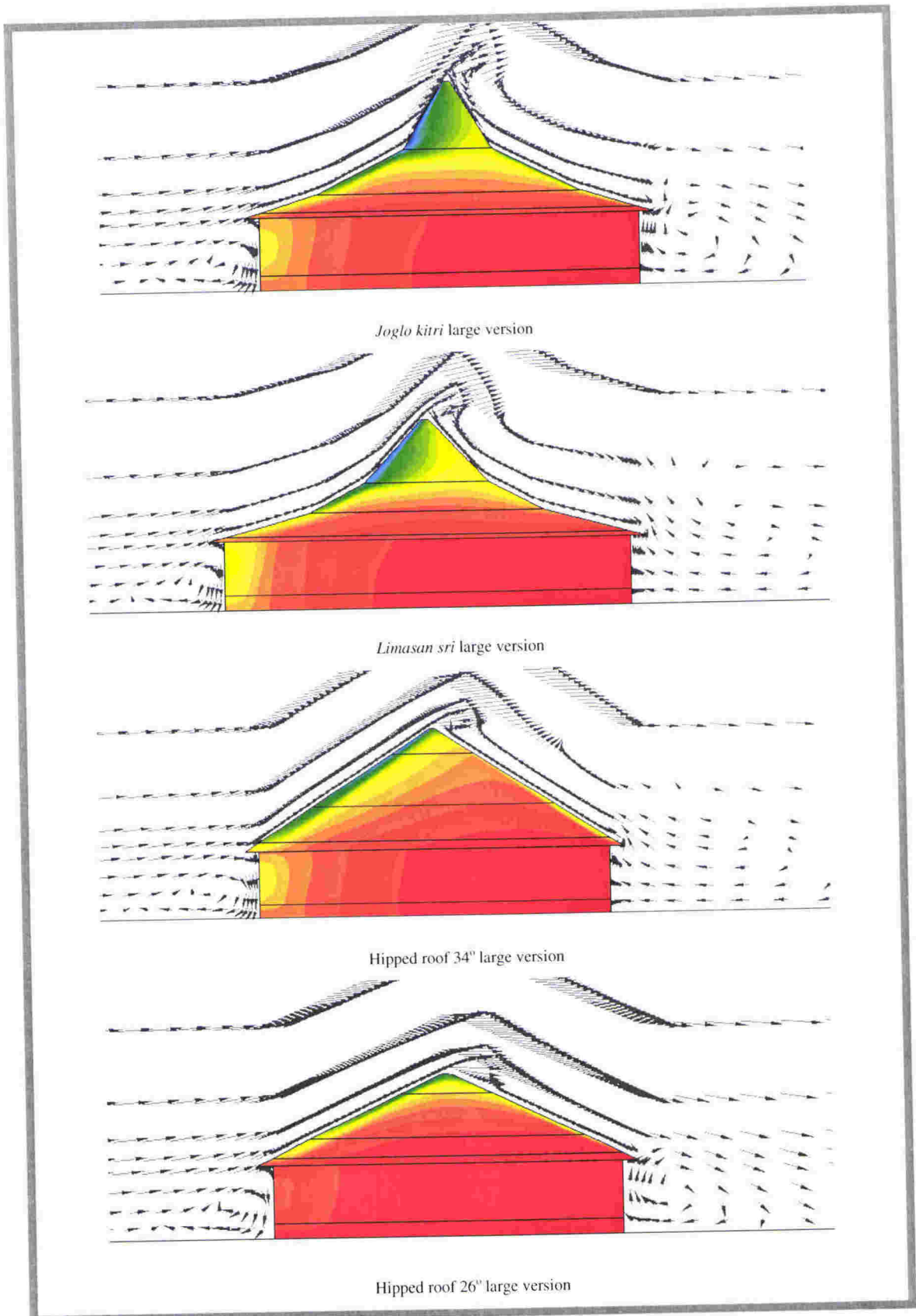
Figure 9-27 Vectors around large version models.
