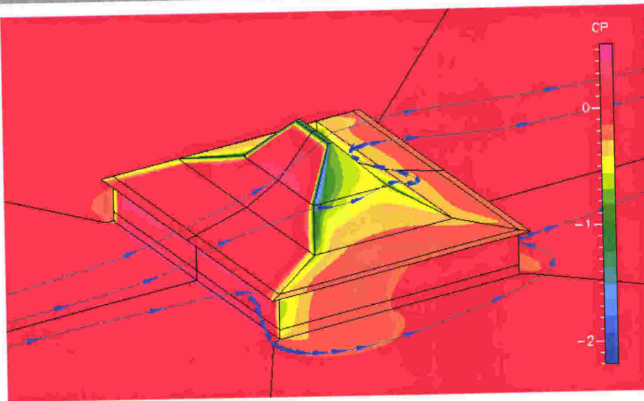
Figure 9-15 Pressure coefficient plot on the surfaces of Limasan sri (L) (front view). Limasan kitri (L) has the same plot with slightly different magnitude.
