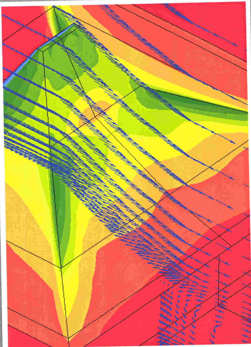
Figure 9-21 Vectors showing the change of airflow from backward flow (behind the guru sector) to forward flow (off the guru sector). Please compare with Figure 9-19.
