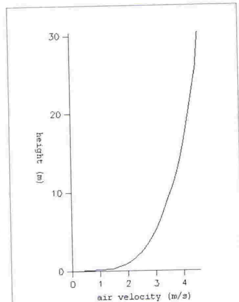
Figure 9-1 Atmospheric boundary layer generated by CFD-ACE to simulate a realistic wind profile around Javanese buildings. It was based on terrain category 3.
