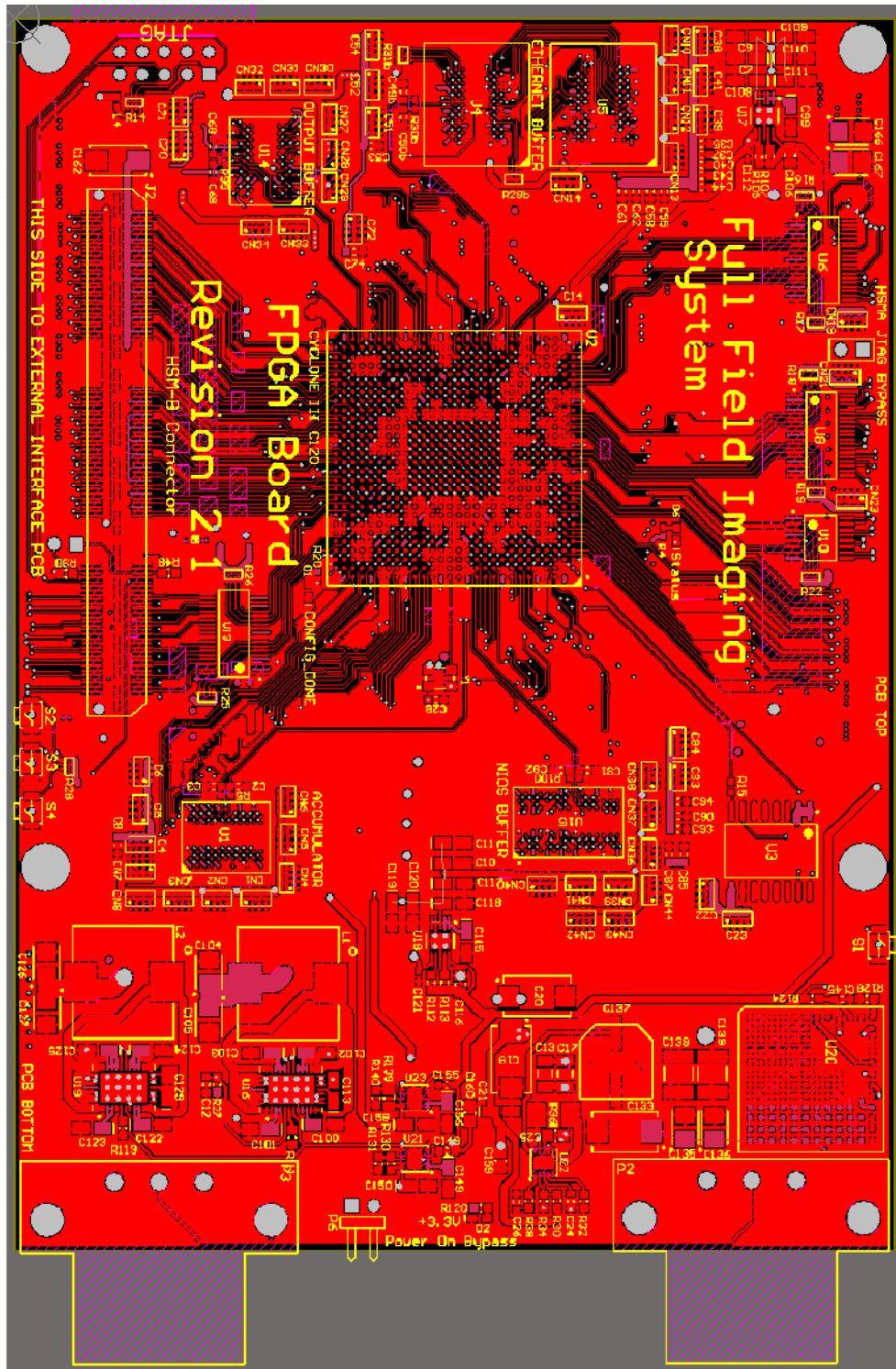
Figure A.2.1 : FPGA Board Rev 2.1 Top Layer
