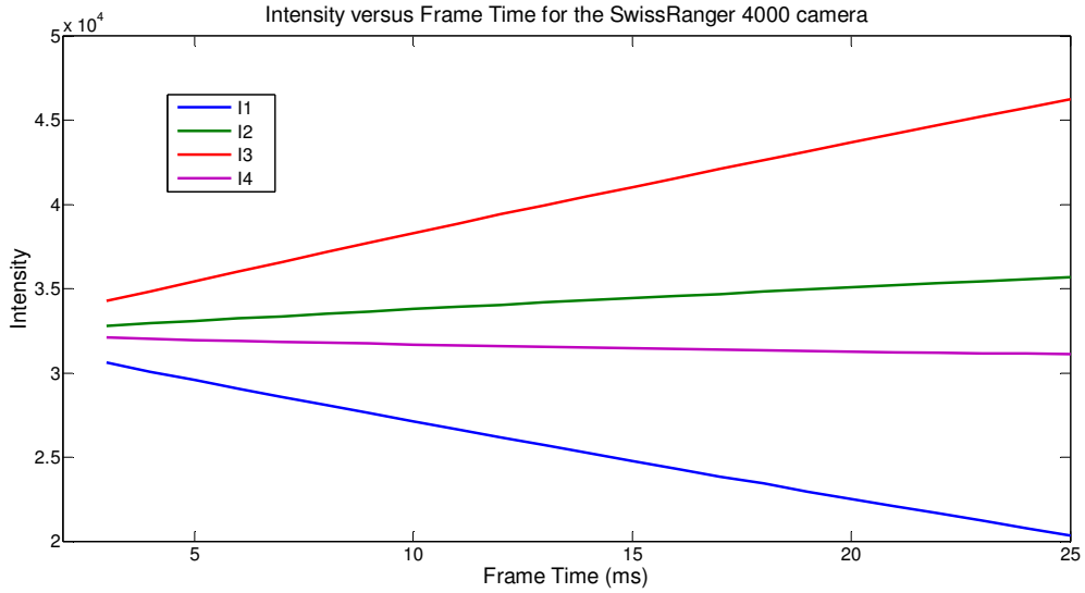
Figure 4.32 Mrasured intensity versus Frame Time for all four frames of the SR-4000 camera
