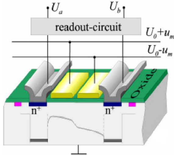
Figure 2.6 Diagram of an indirect time of flight pixel (Ringbeck & Hagebecker, 2007)
