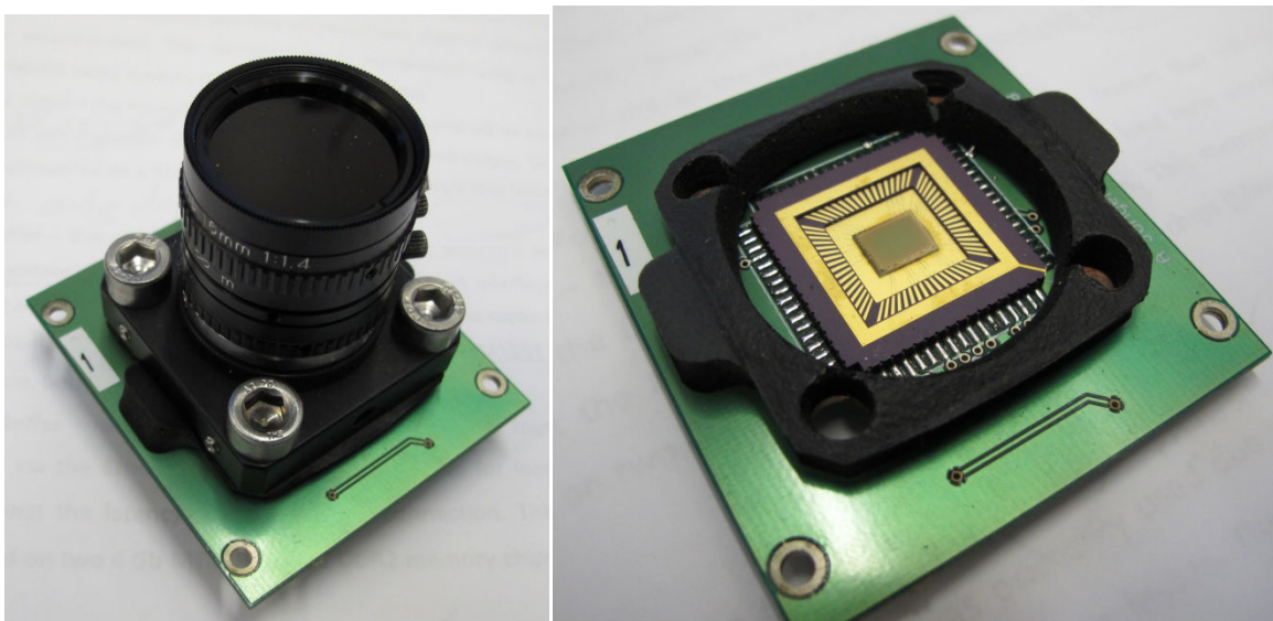
Figure 3.2 Optical lens assembly photograph (left) and sensor IC (right)
