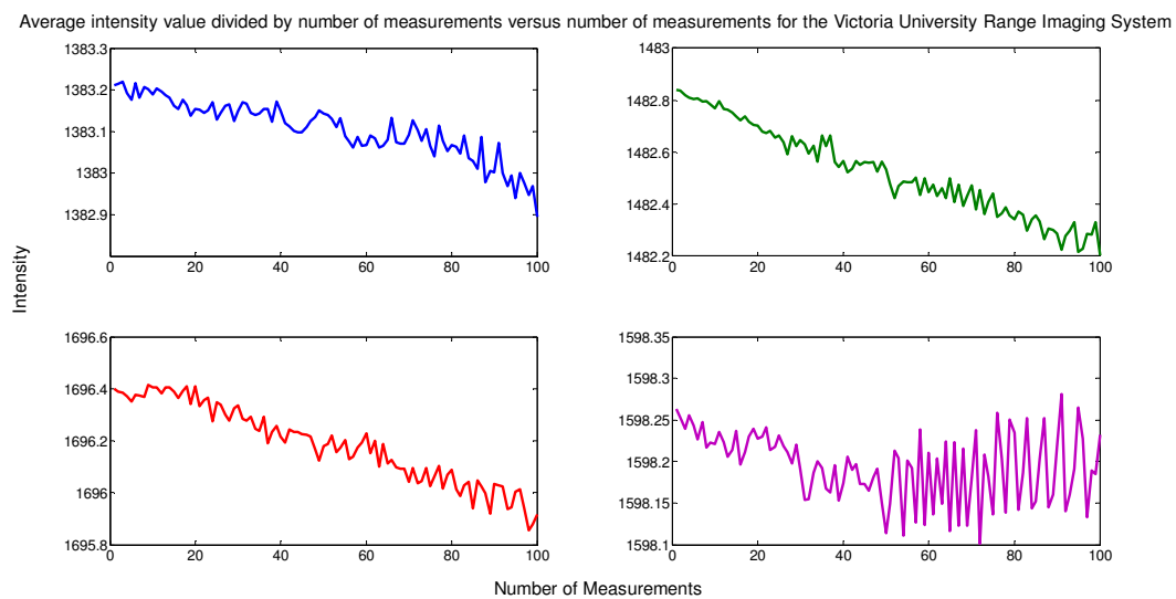
Figure 4.23 Average intensity value versus number of measurements for the Victoria University Range Imaging System
