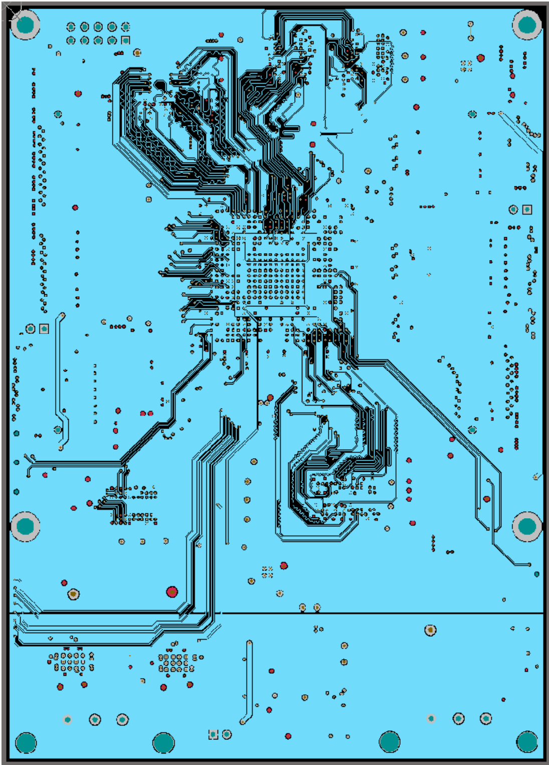
Figure A.2.3 : FPGA Board Rev 2.1 Mid Layer 2
