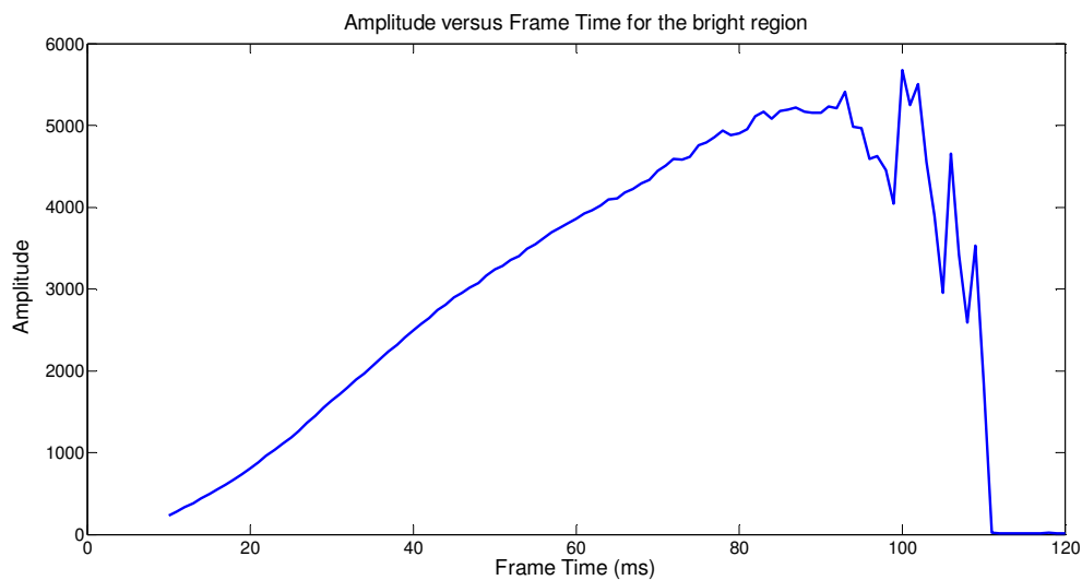
Figure 4.5 Measured Intensity of all four frames versus Frame Time for the bright region
