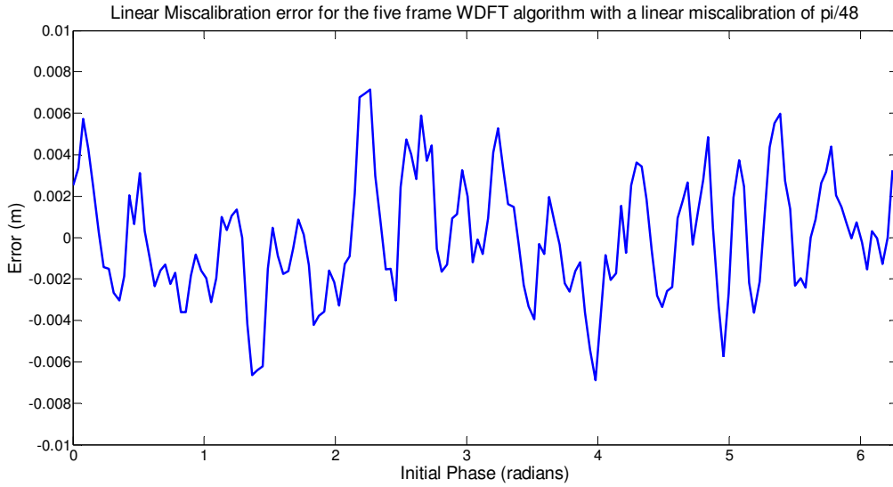
Figure 5.41 Linear miscalibration error for the five frame WDF algorithm
