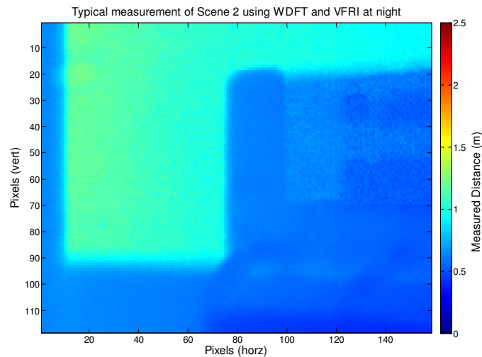
Figure 6.11 Typical measurement of Scene 2 using the WDFI + VFRI system at night
