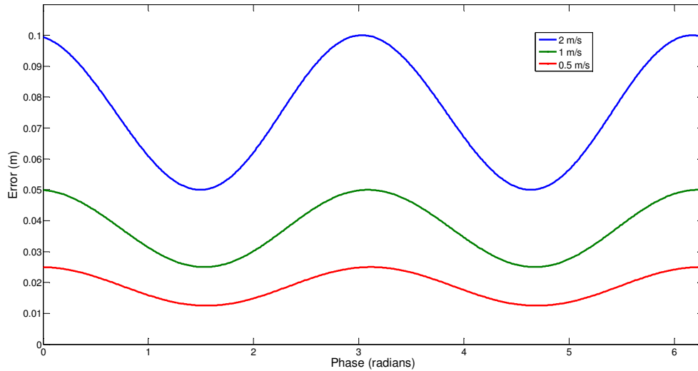
Theoretical error from axial motion for various speeds using 30 MHz modulation, 25 ms frame time and 4 frames per measurement
