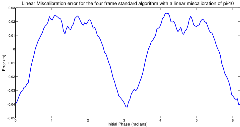
Figure 5.11 Linear miscalibration error for the four frame standard algorithm with a linear miscalibration of \pi/40
