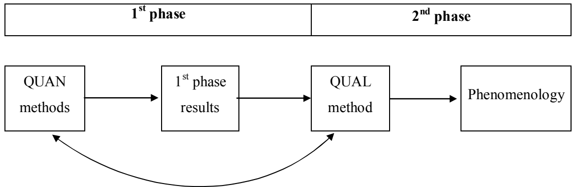
Figure 3.1.: Research design
