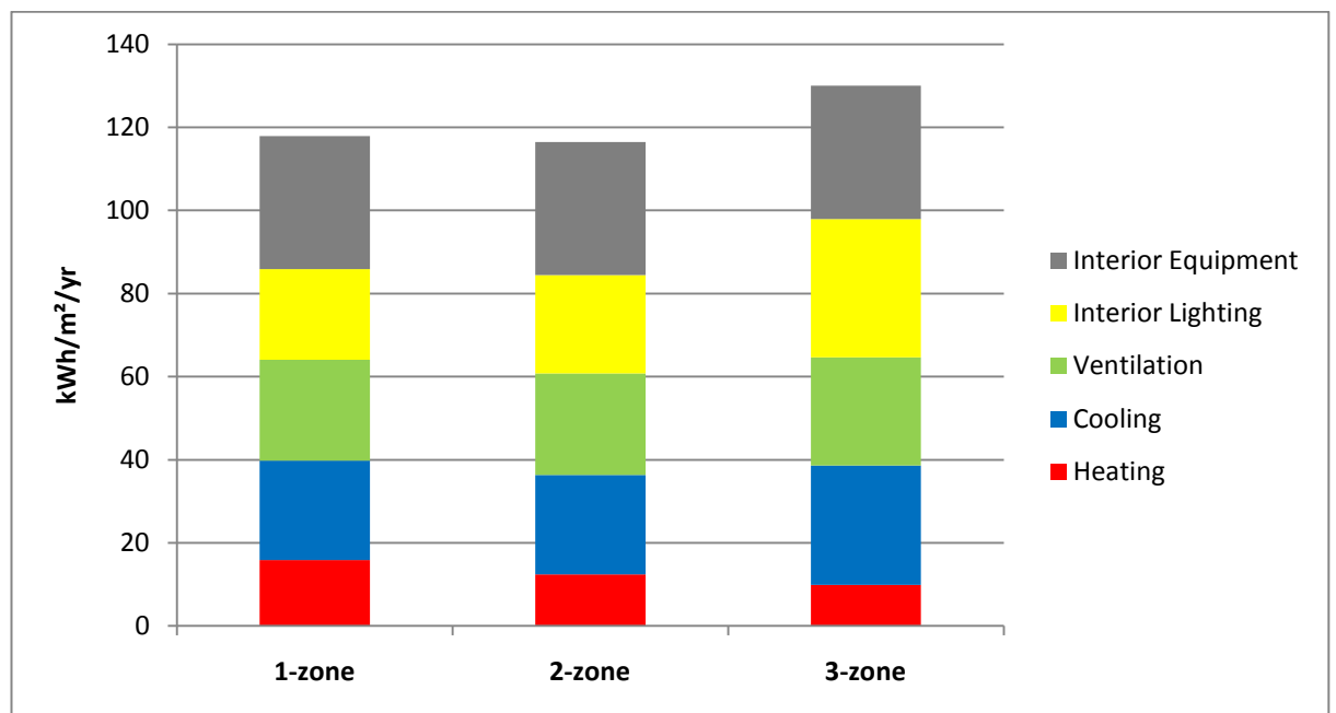
Figure 40 – Mixed Mode with daylight control simulations
