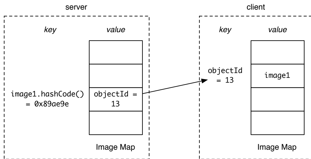
Figure 5.2: Example object map for images. On the server image1 indexes to the integer 13 in the object map. This value is then used to index the object map on the client, hence image1 is stored.
